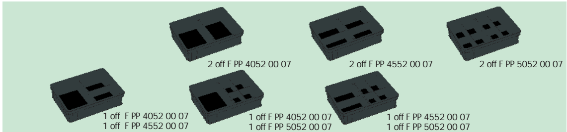
Art. F PP 4052 00 07 with one partition mm 256x178x90h
