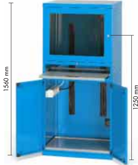
Dim. 717x635x1560 mm h. Complete with: 2 height-adjustable shelves, 1 retractable keyboard shelf.
